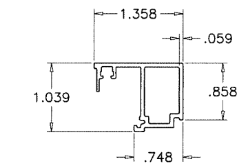
3A GLASS STOP (S77)
