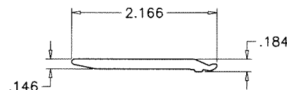
4A GLASS SUPPORT (S77)
