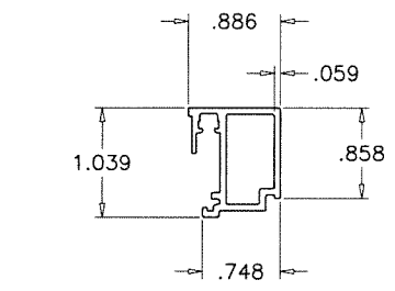
3 GLASS STOP (S67)
