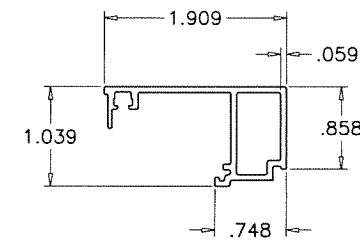
3B GLASS STOP (S91)
