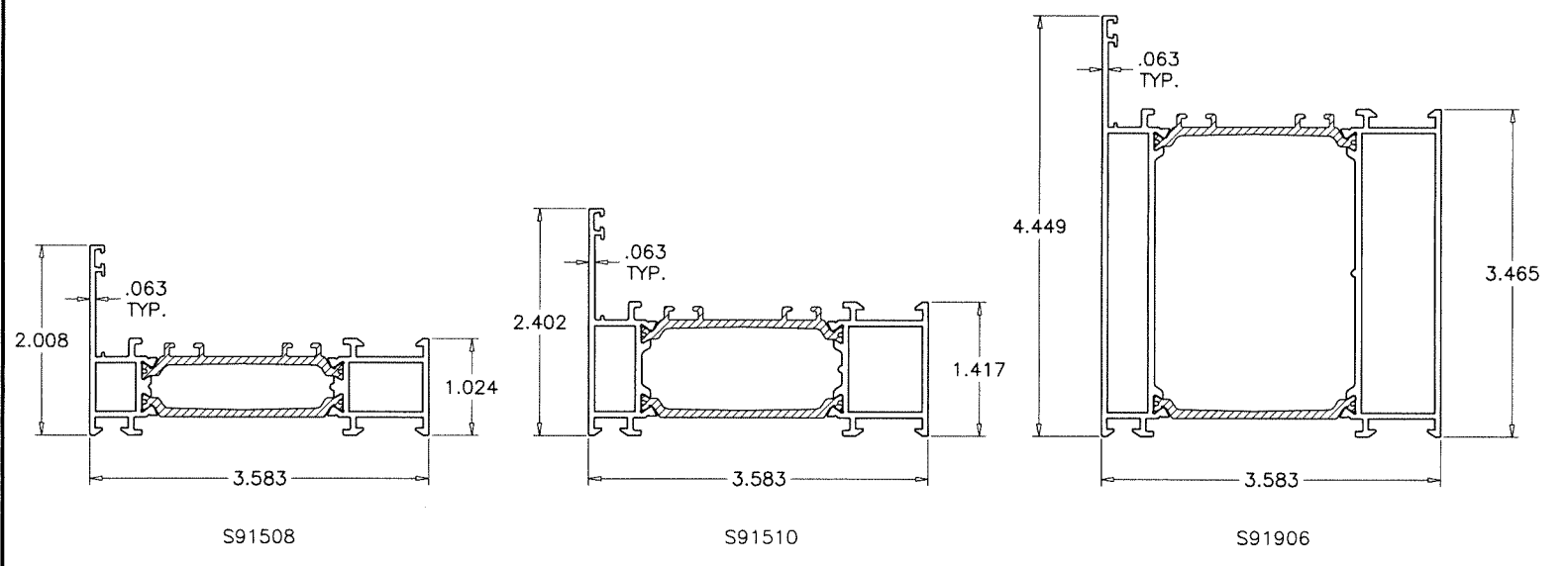
①B WINDOW FRAMES (S91)
